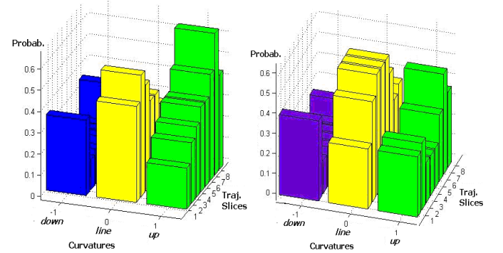
Fig.9. The left image represents the Top-Grasping Learning Table P(C/GD) . The probability of the curvature down varies between 0.14 and 0.35 along the trajectory slices. The probability of line varies between 0.16 and 0.57. The probability of curvature up varies between 0.19 and 0.66. The right image represents the Side-Grasping Learning Table P(C/GD) . The probability of curvature down varies between 0.16 and 0.4. The probability of line varies between 0.3 and 0.6. The probability of curvature up varies between 0.2 and 0.5. The sum of the down , line and up in each slice must be 1.
