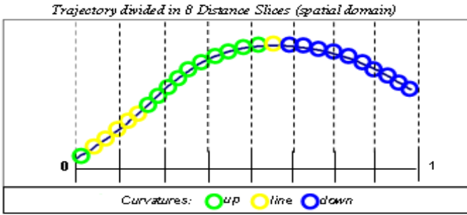
Fig.5. Example of a trajectory divided into 8 equal slices. At each slice can be found N curvatures between UP, DOWN and LINE (no curvature). The Probability of each type of curvature is computed at each slice.
